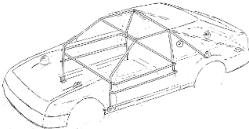
MAXIMUM SPECIFICATION ROLL CAGE
